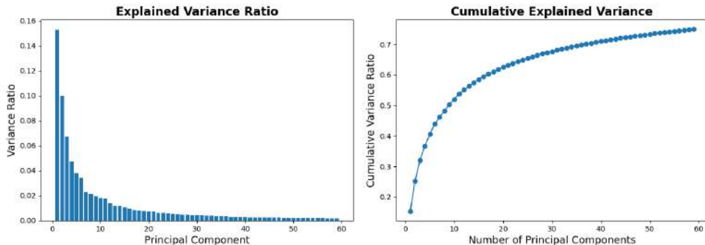
Figure 3: Explained variance ratio for each principal component (left) and cumulative explained variance (right). In total, at least 75% of the variance is explained after PCA.
