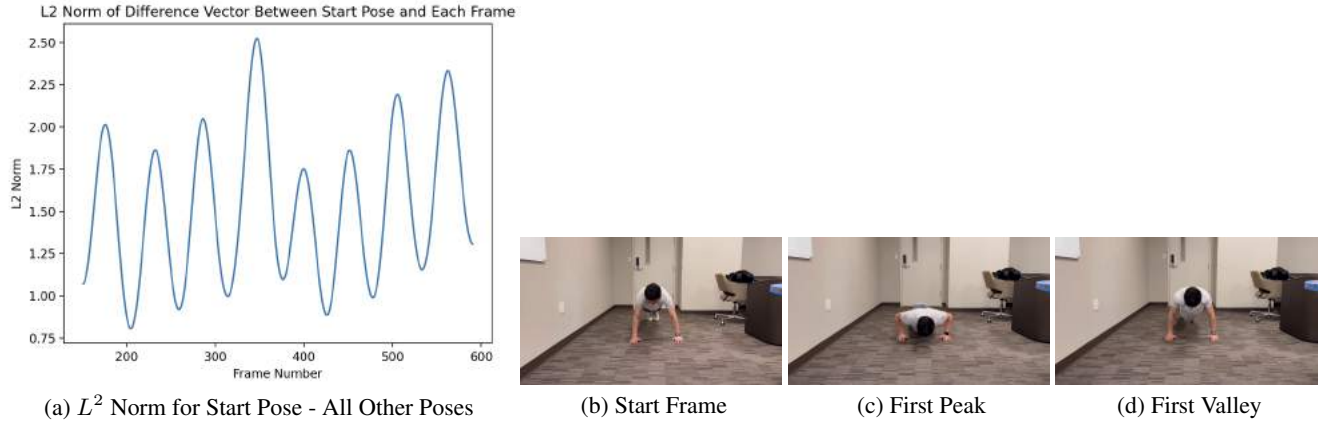
Figure 6: L^2 Norm Graph & Start, Peak, and Valley Frames for the Good Pushup Video
