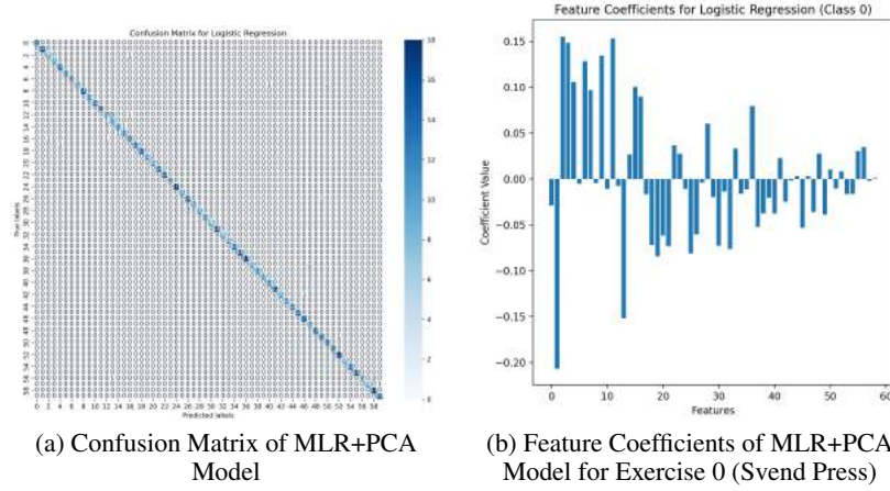
Figure 5: Confusion Matrix & Feature Coefficients of MLR+PCA model
